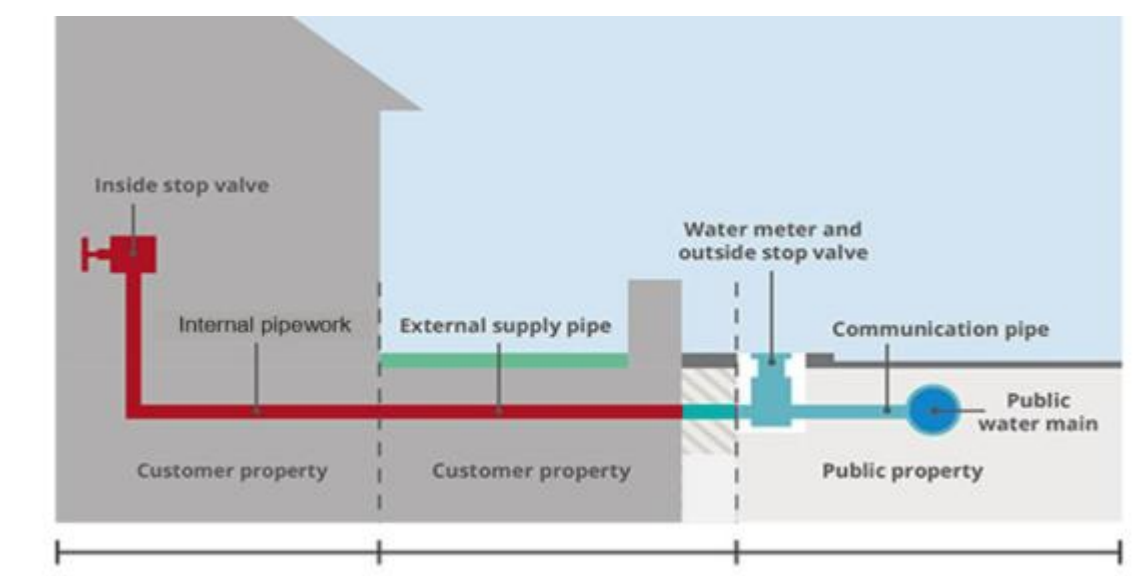
Figure 3.3 Typical layout of a Connection's pipework
